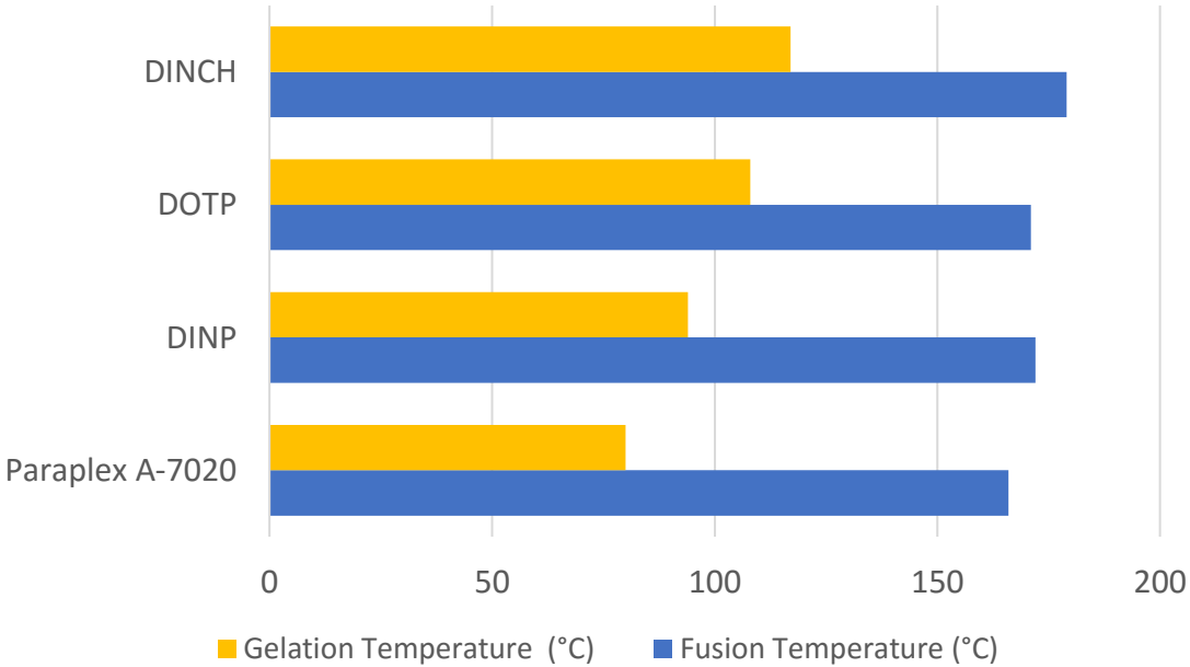
Gelation/Fusion Temperature
